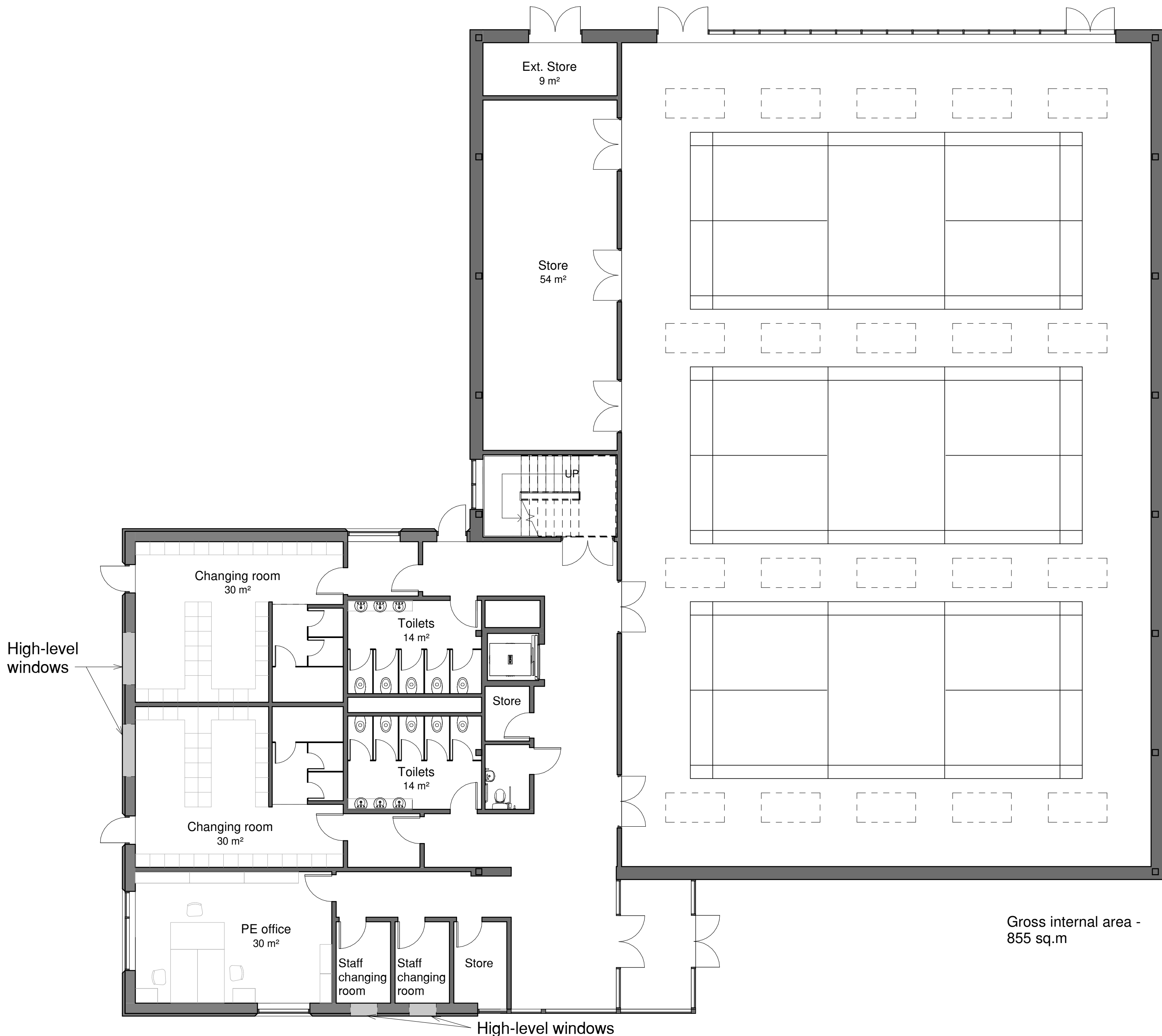
1 Proposed Ground Floor Plan 1 : 100
